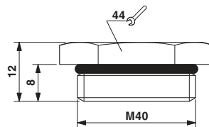
Filler plugs M40
