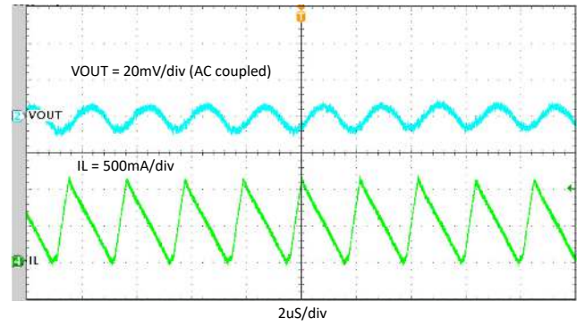
Figure 10-15. Steady State, I_{OUT} = 0.5 A
