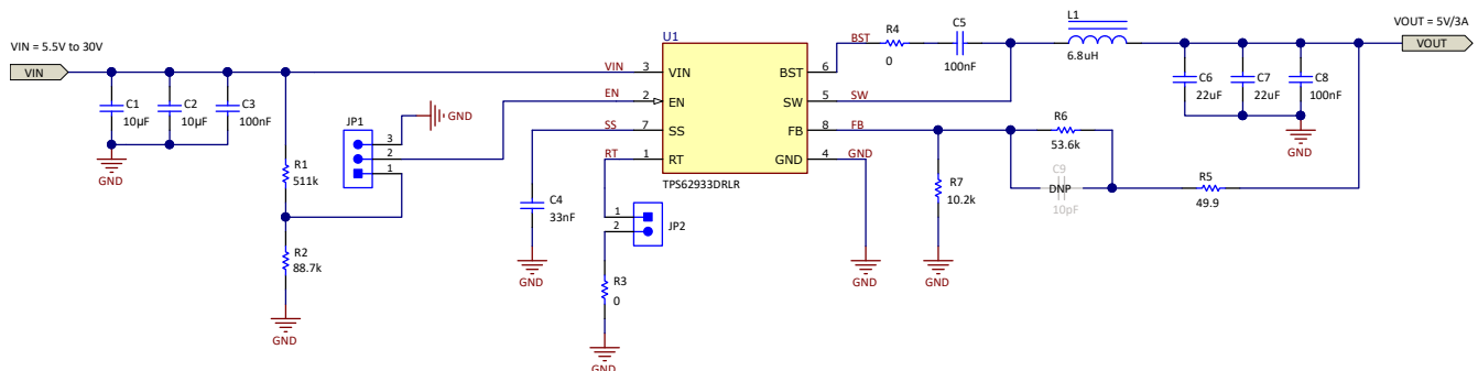
Figure 10-1. TPS62933 5-V Output, 3-A Reference Design
