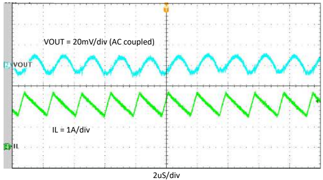
Figure 10-17. Steady State, I_{OUT} = 2 A
