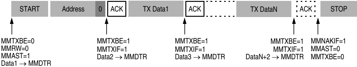
(b) Master Receive Mode
