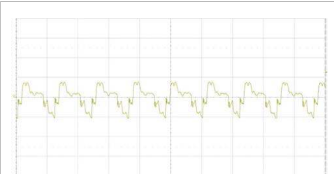
Output voltage ripple at: T_{P1} = +25^{\circ}\text{C} , V_I = 48\text{ V} , I_o = 15\text{ A} resistive load. Trace: output voltage (20 mV/div.). Time scale: (2 \mu\text{s} /div.). 20 MHz bandwidth.
