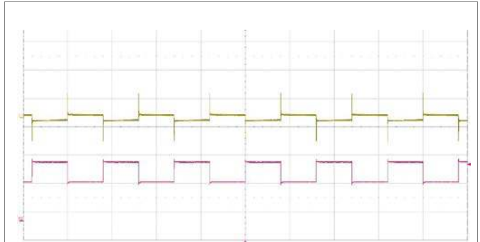
Output voltage response to load current step- change (7.5-11.25-7.5 A) at: T_{P1} = +25^{\circ}\text{C} , V_I = 48\text{ V} . Top trace: output voltage (500 mV/div.). Bottom trace: load current (5 A/div.). Time scale: (10 ms/div.).
