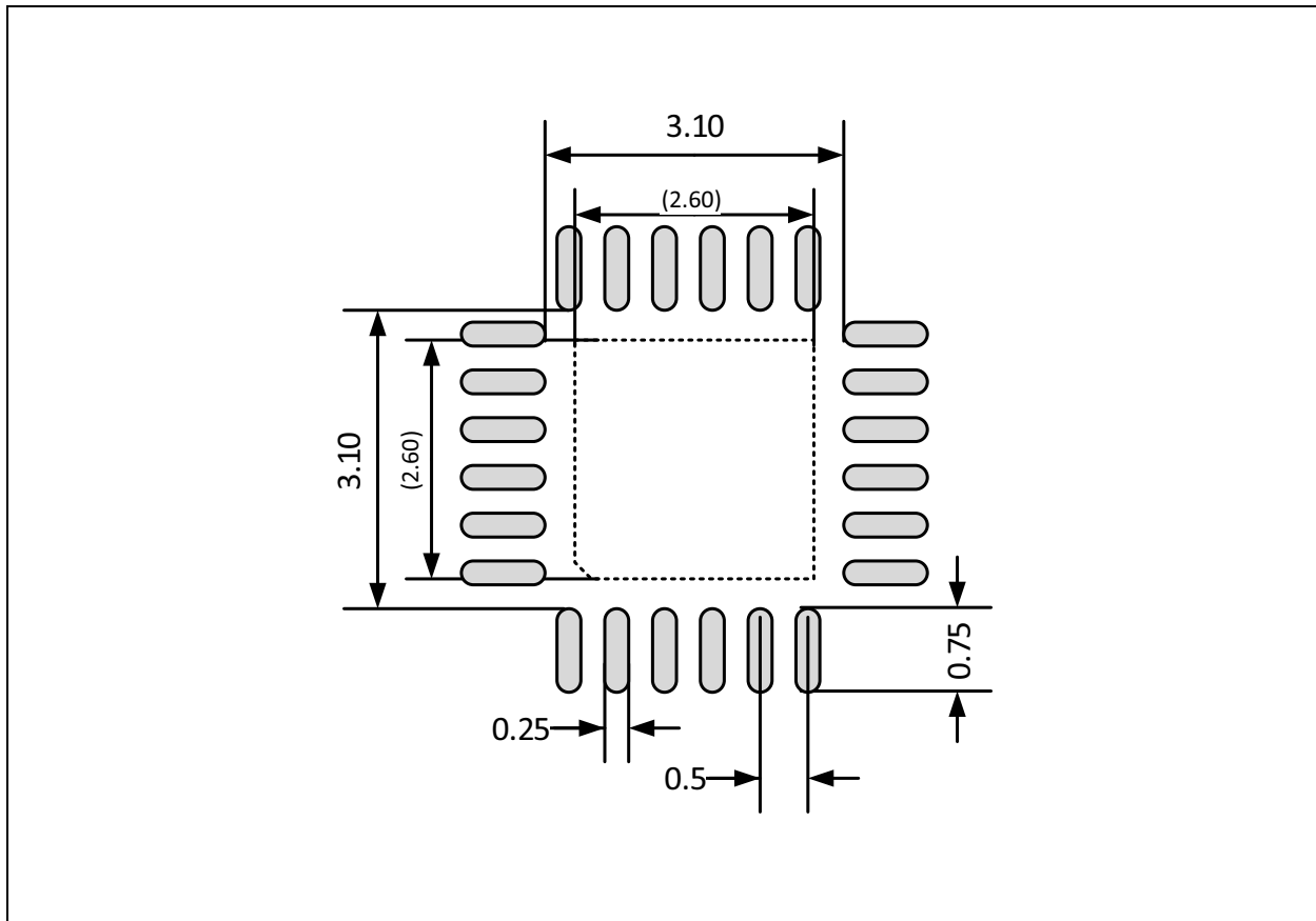
Figure 140: Landing Pattern
