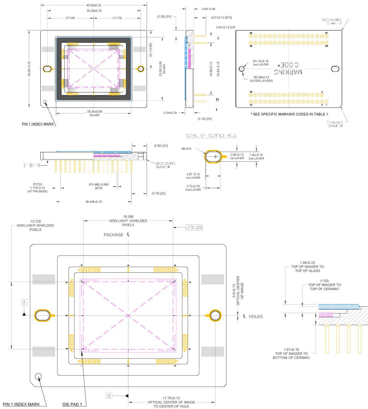
Figure 24. Completed Assembly
