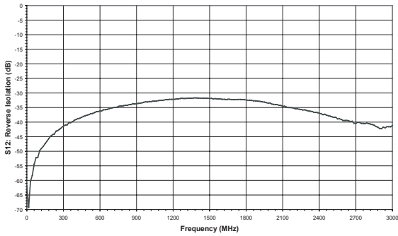
Figure 5: Reverse Isolation (S12) vs. Frequency (T C = +25 °C, V DD = +5 V, V AGC = +3 V)
