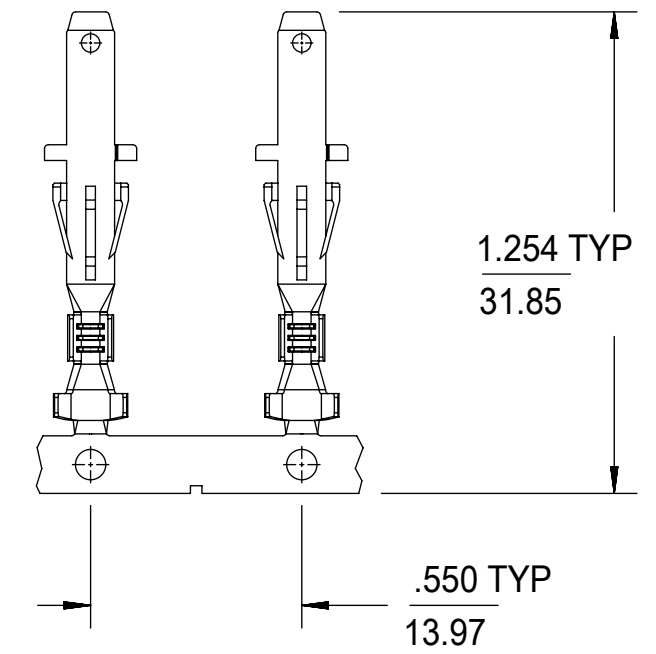
CARRIER STRIP PROGRESSION SCALE 2:1
