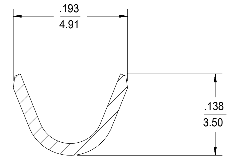
SECTION V-V SCALE 10:1 INSULATION CRIMP
