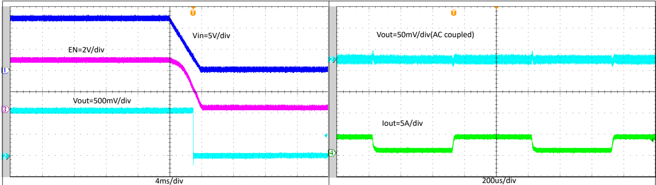
Figure 8-14. Start-Up with V_{IN} Falling, I_{OUT} = 4 A
