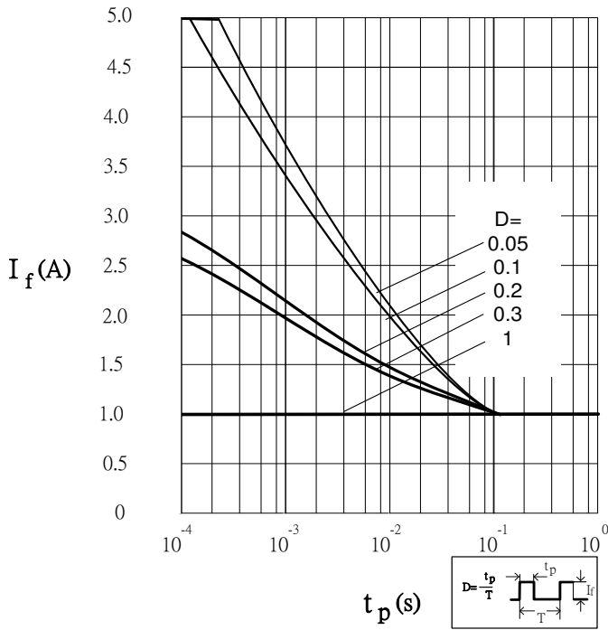
Operating Range of Pulse Currents ( I_f vs. t_p , T_a=25^\circ\text{C} , "D" means Duty cycle)
