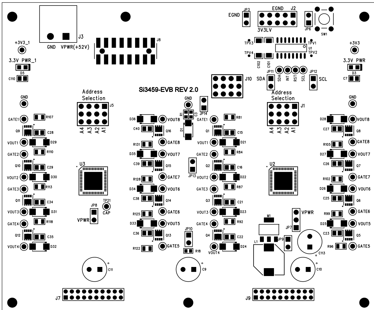
Figure 20. Evaluation Board Top Silkscreen
