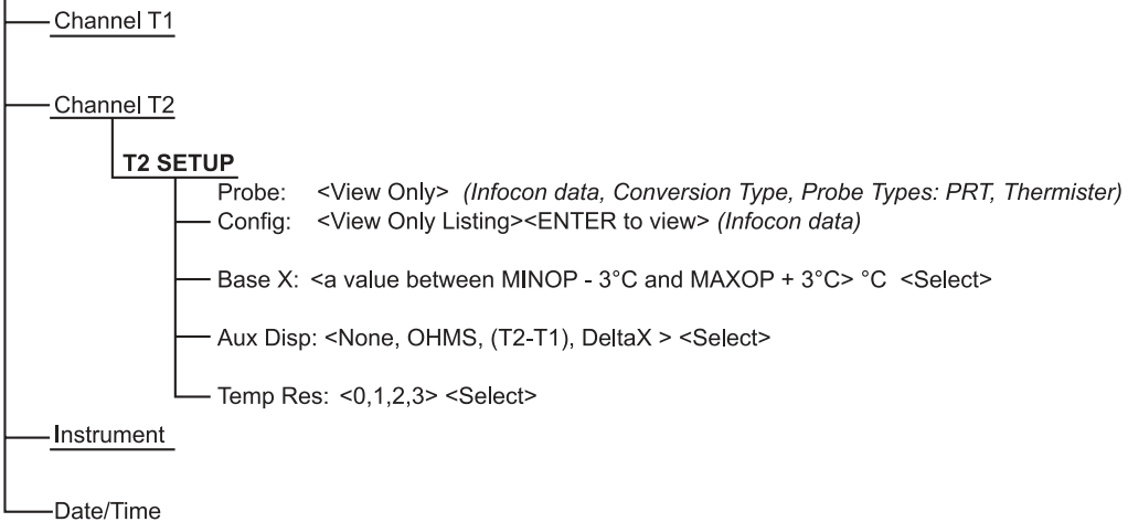
Figure 10 1524 Menu (cont)
