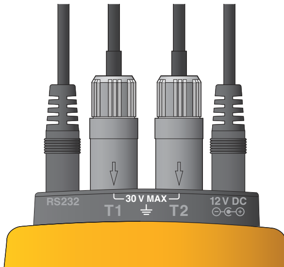
Figure 4 Input/Output Connections - 1524
