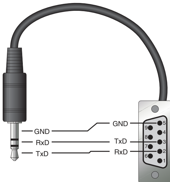
Figure 17 RS-232 wiring
