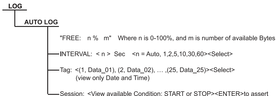
Figure 14 1524 Menu (cont)
