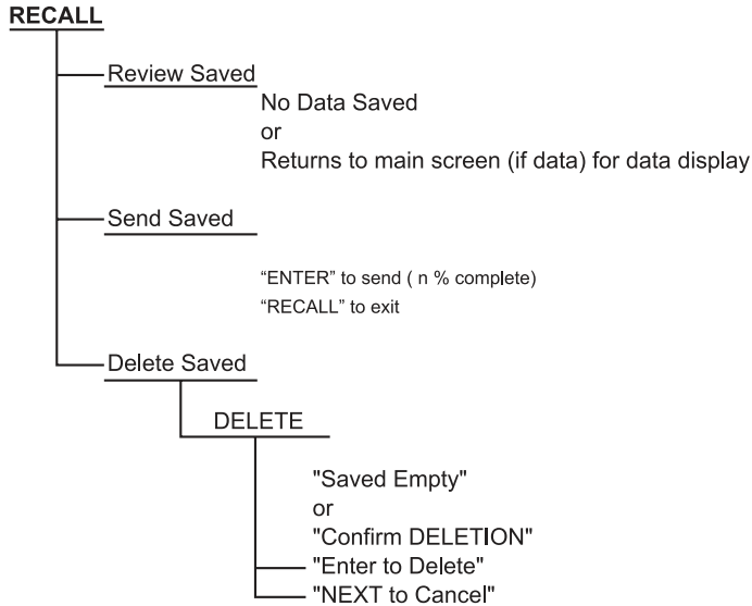
Figure 8 1523 Menu (cont)
