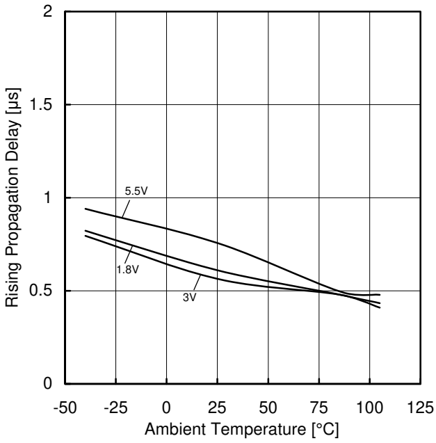
Figure 43. Rising Propagation Delay vs Ambient Temperature ( C_L=15pF , 100mV Overdrive)
