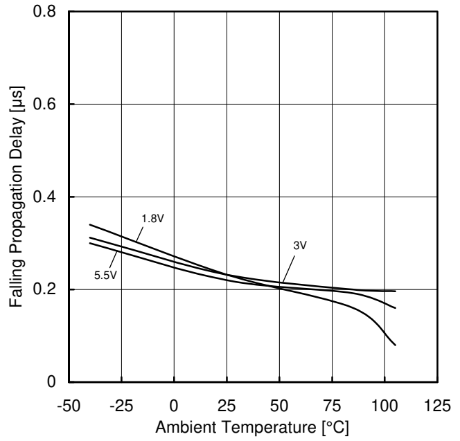
Figure 44. Falling Propagation Delay vs Ambient Temperature ( C_L=15pF , 100mV Overdrive)
