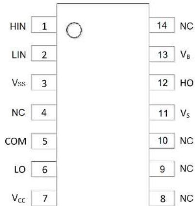
Top View SO-14
