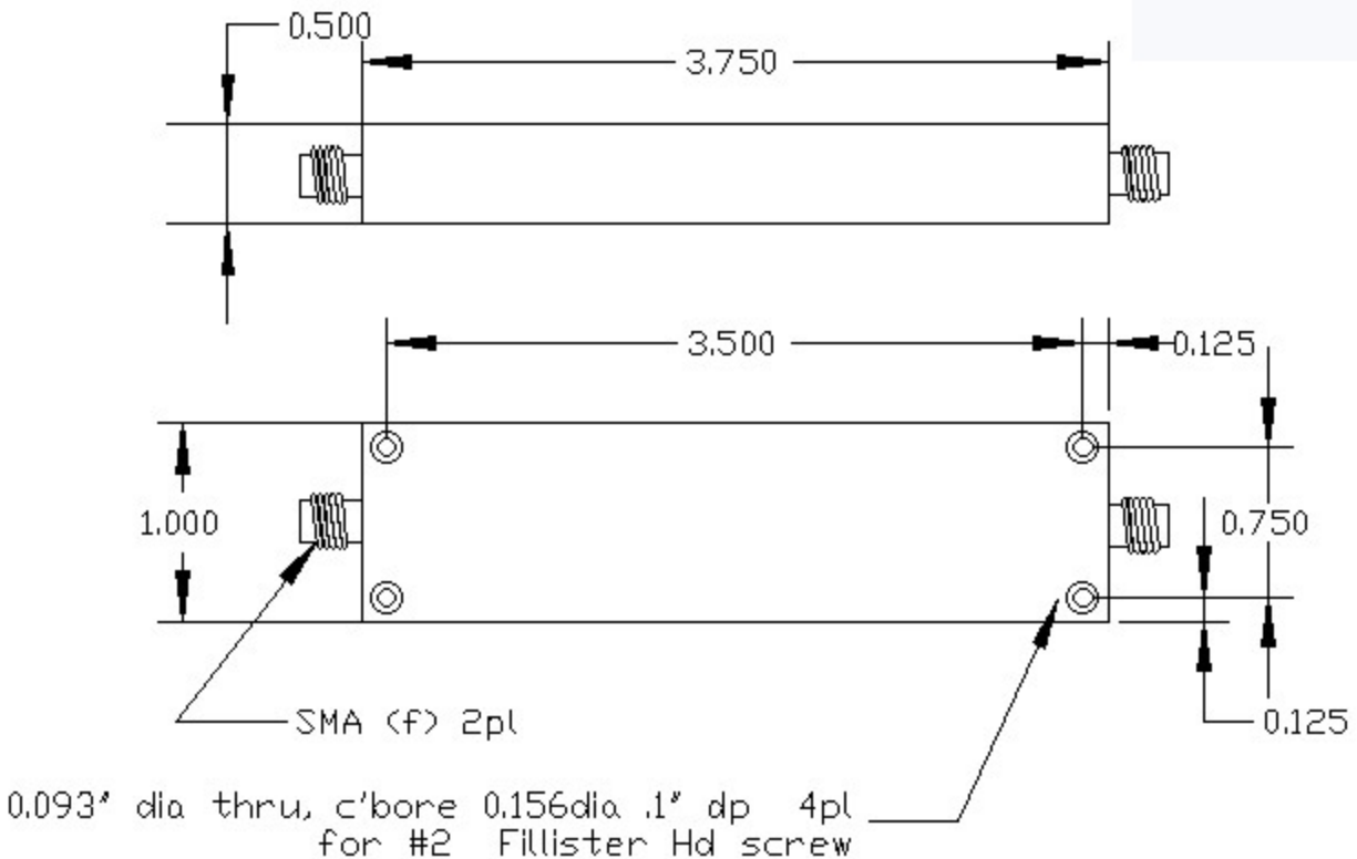
Outline Drawing 986187
