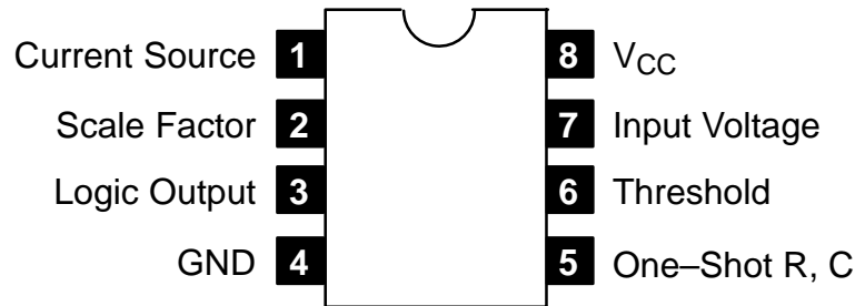
Pin Connection Diagram
