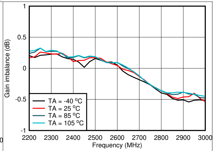
Figure 14. Gain Imbalance vs Frequency and Temperature
