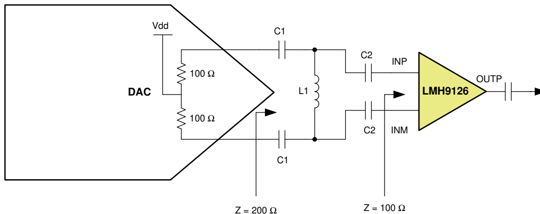
Figure 19. LMH9126 Driven by a DAC With 200-Ω Termination
