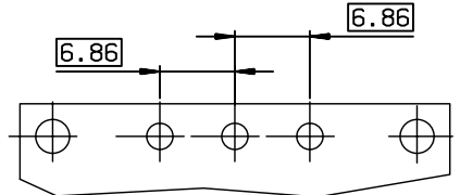
LAYOUT DIMENSIONS (after plating) CONNECTOR SIDE VIEW
