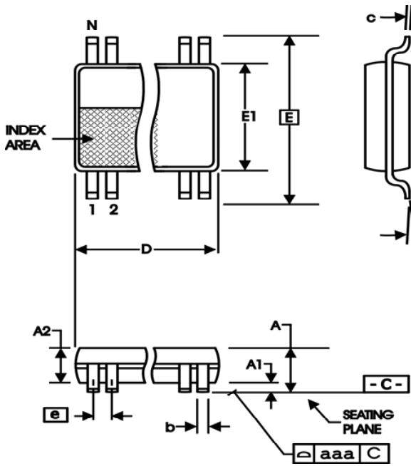
PACKAGE OUTLINE - G SUFFIX FOR 48 LEAD TSSOP
