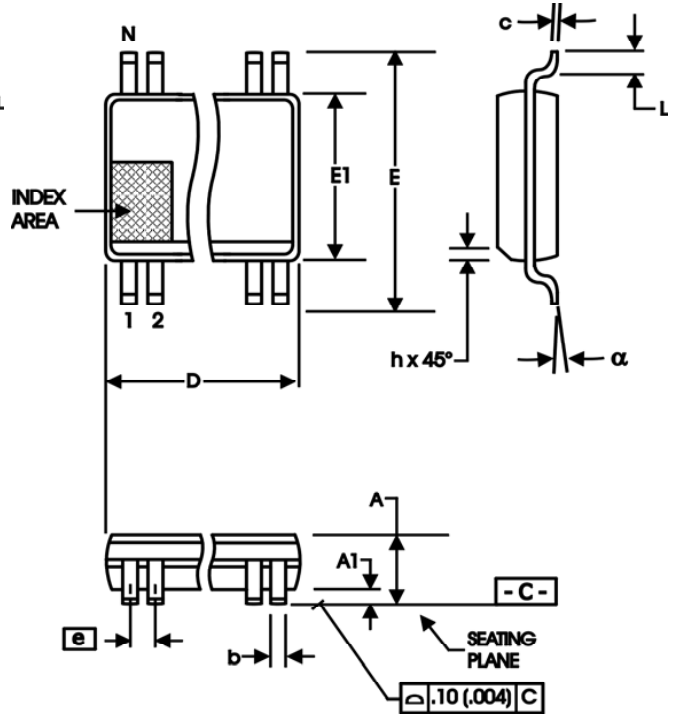
PACKAGE OUTLINE - F SUFFIX FOR 48 LEAD SSOP
