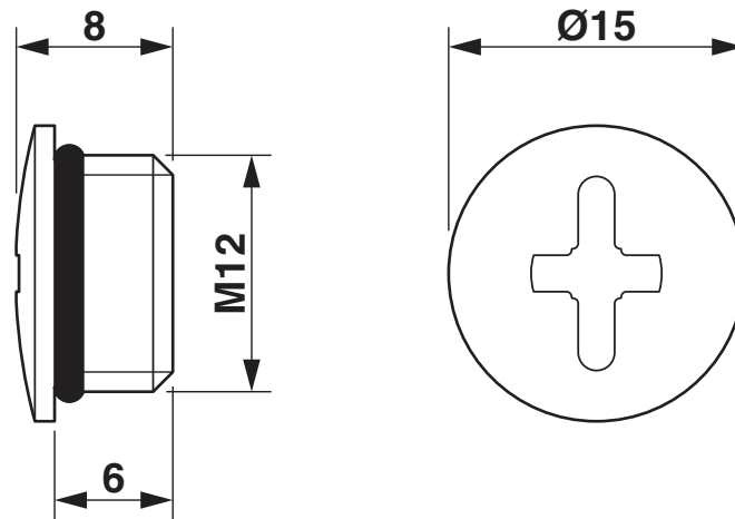
Dimensional drawing
