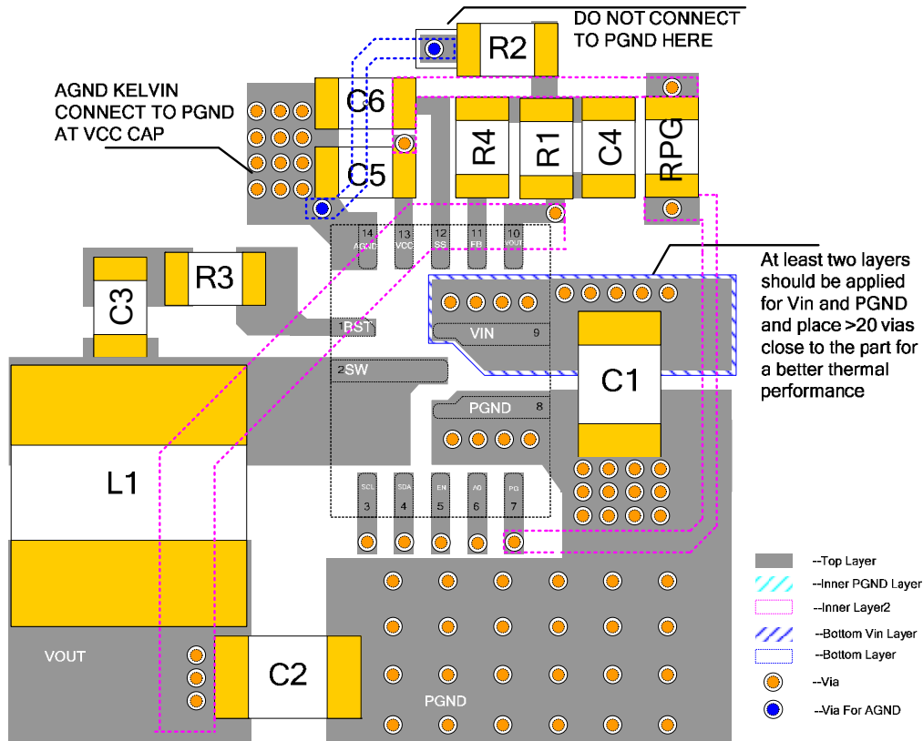
Figure 14: Recommended Layout
