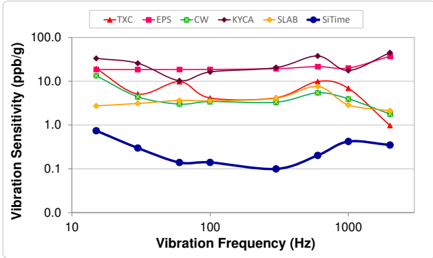
Figure 19. Vibration Robustness [5]
