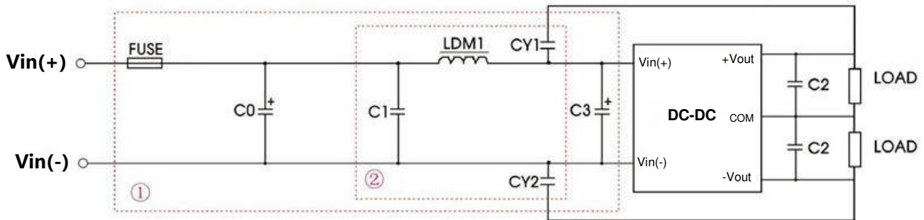
Figure 6. EMC Recommended Circuit
