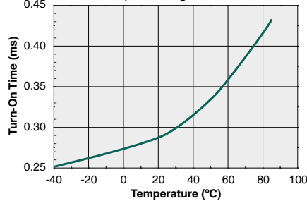
Typical Turn-On Time vs. Temperature ( I_F=5mA , I_L=80mA )
