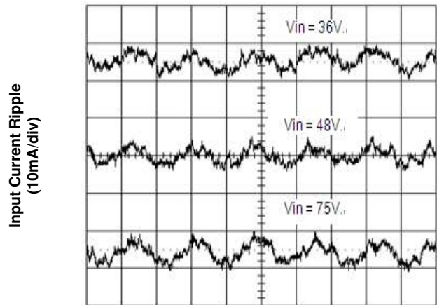
Figure 4. Input Reflected Ripple Current at Full Load
