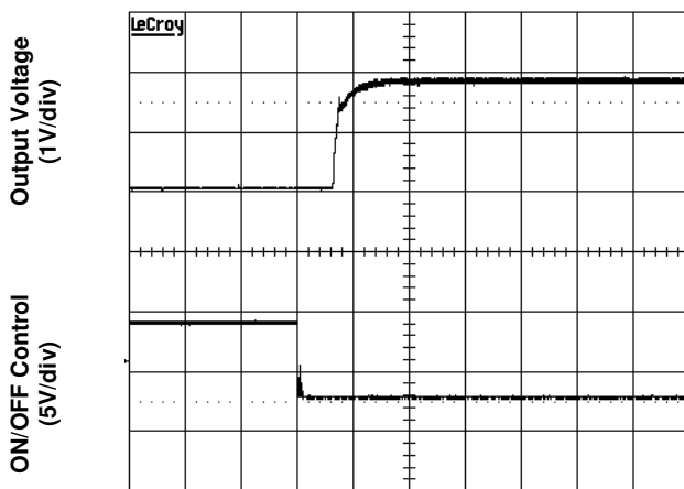
Figure 5. Start-Up from Enable Control (typical Vin, zero load)
