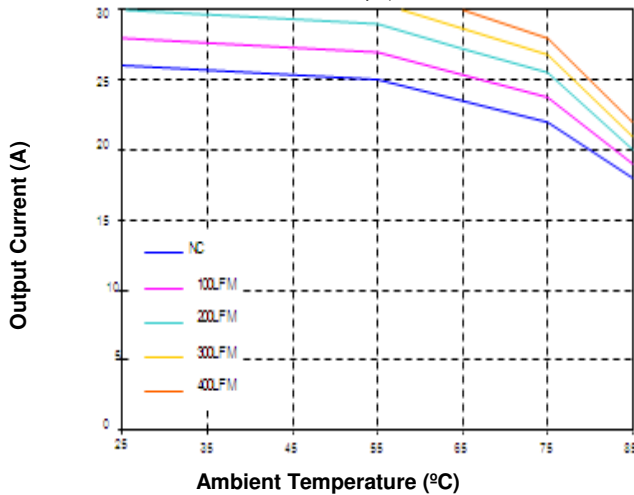
Figure 9. Current Derating Curve with Open Frame (Direction 3 (Ref. Figure 10); typical Vin, unit soldered onto a fixture board)
