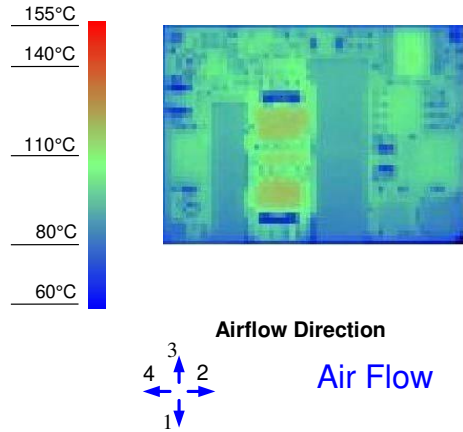
Figure 10. Thermal Image for Airflow Direction 3 (25A output, 55°C ambient, 0 LFM, typical Vin, open frame, unit soldered onto a fixture board)
