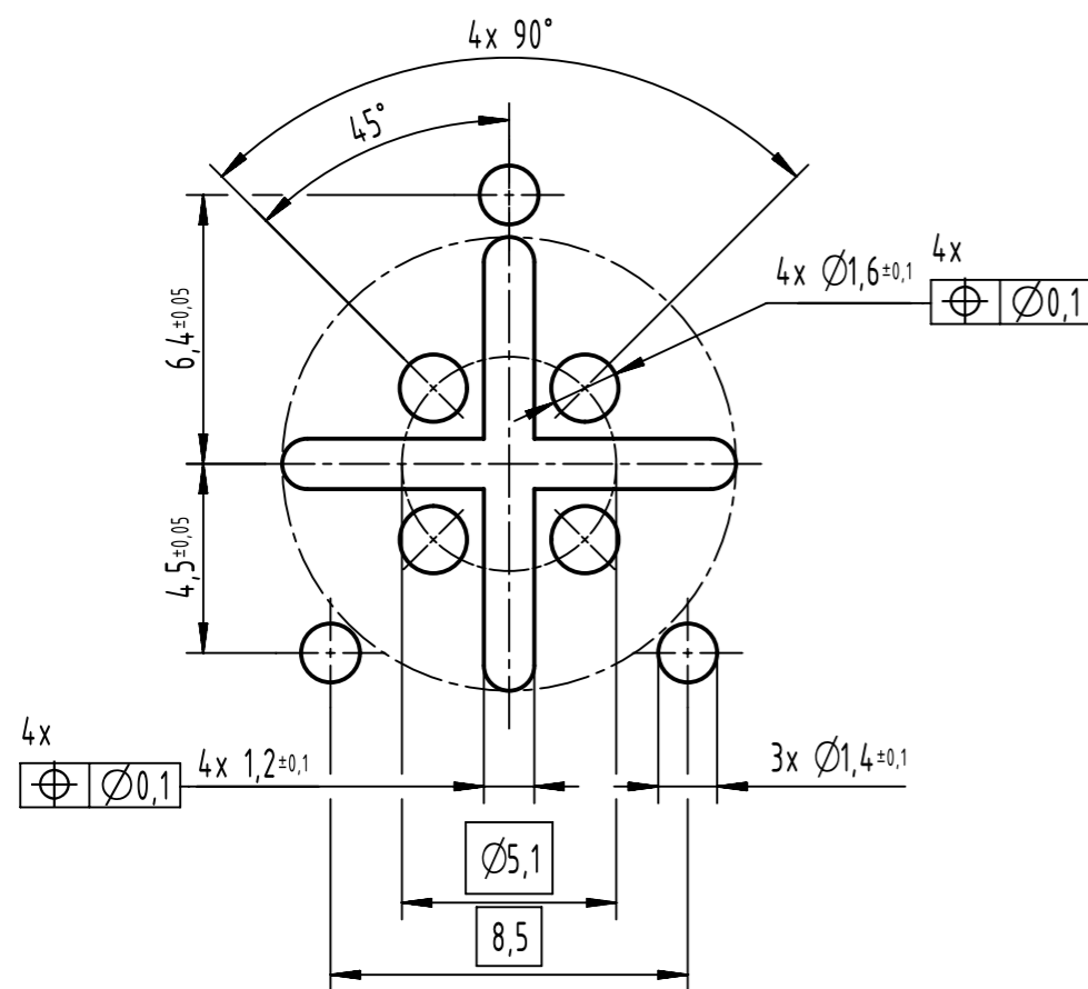
recommended PCB-layout (5:1)
