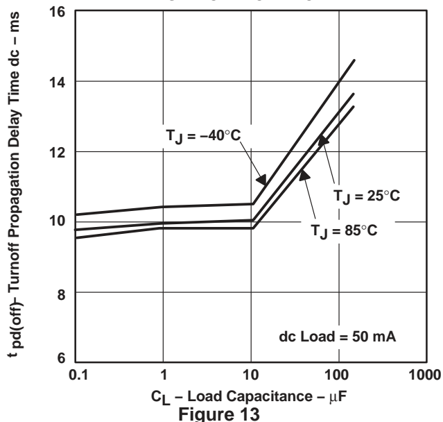
TURNOFF PROPAGATION DELAY TIME dc 12-V xVPP SWITCH VS LOAD CAPACITANCE
