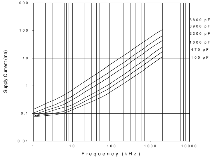
Fig. 12 Supply Current vs. Frequency Vcc = 8V
