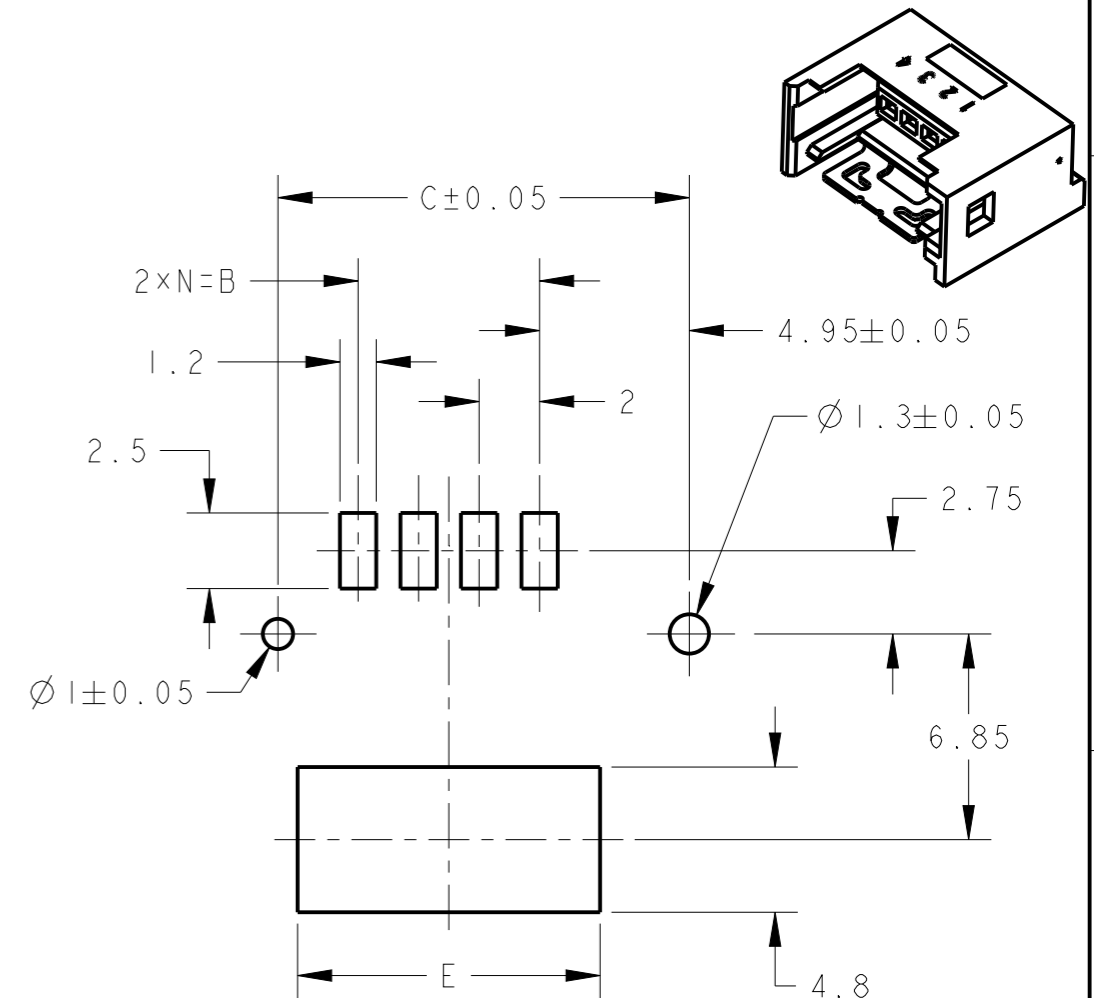
REFERENCE DIMENSION OF PCB(MOUNTING SIDE)
