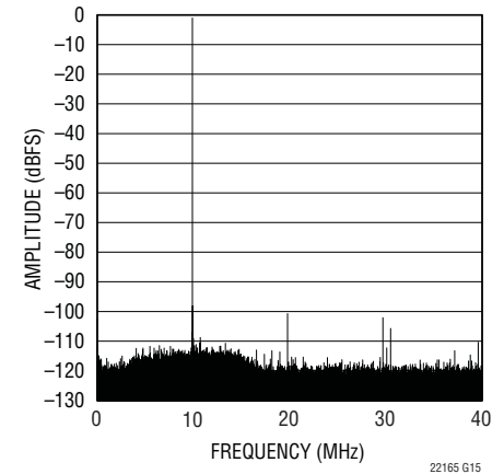
LTC2216 64k Point FFT, f_{IN} = 70.2\text{MHz} , -1\text{dBFS}
