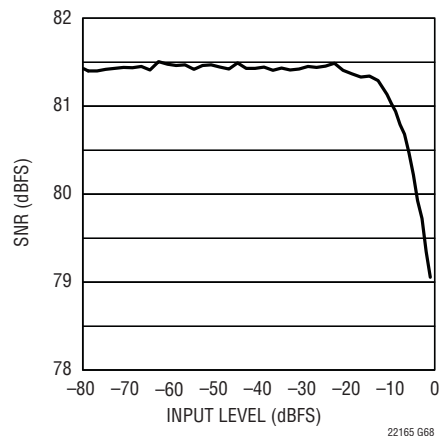
LTC2215 SNR vs Input Level, f_{IN} = 140.5\text{MHz}
