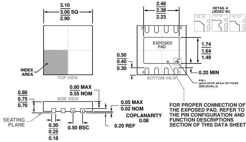
Figure 81. 8-Lead Lead Frame Chip Scale Package [LFCSP] 3 mm x 3 mm Body and 0.75 mm Package Height (CP-8-5) Dimensions shown in millimeters
