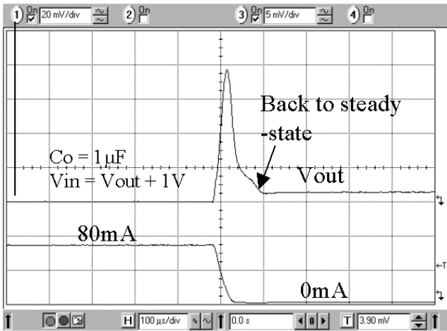
Figure 15. Load Transient Improvement Effect
