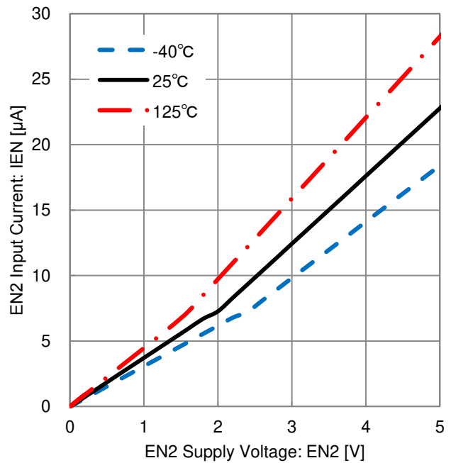
Figure 21. EN2 Input Current vs EN2 Supply Voltage (EN2 Inflow Current)
