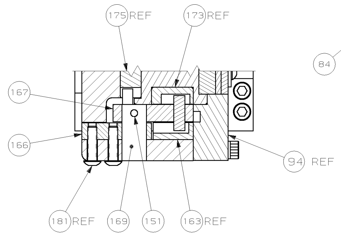
DETAIL K SCALE 2:1
