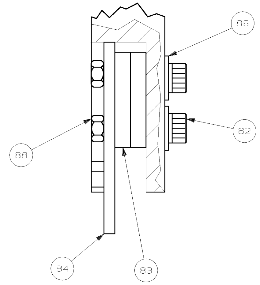
DETAIL K SCALE 2:1
