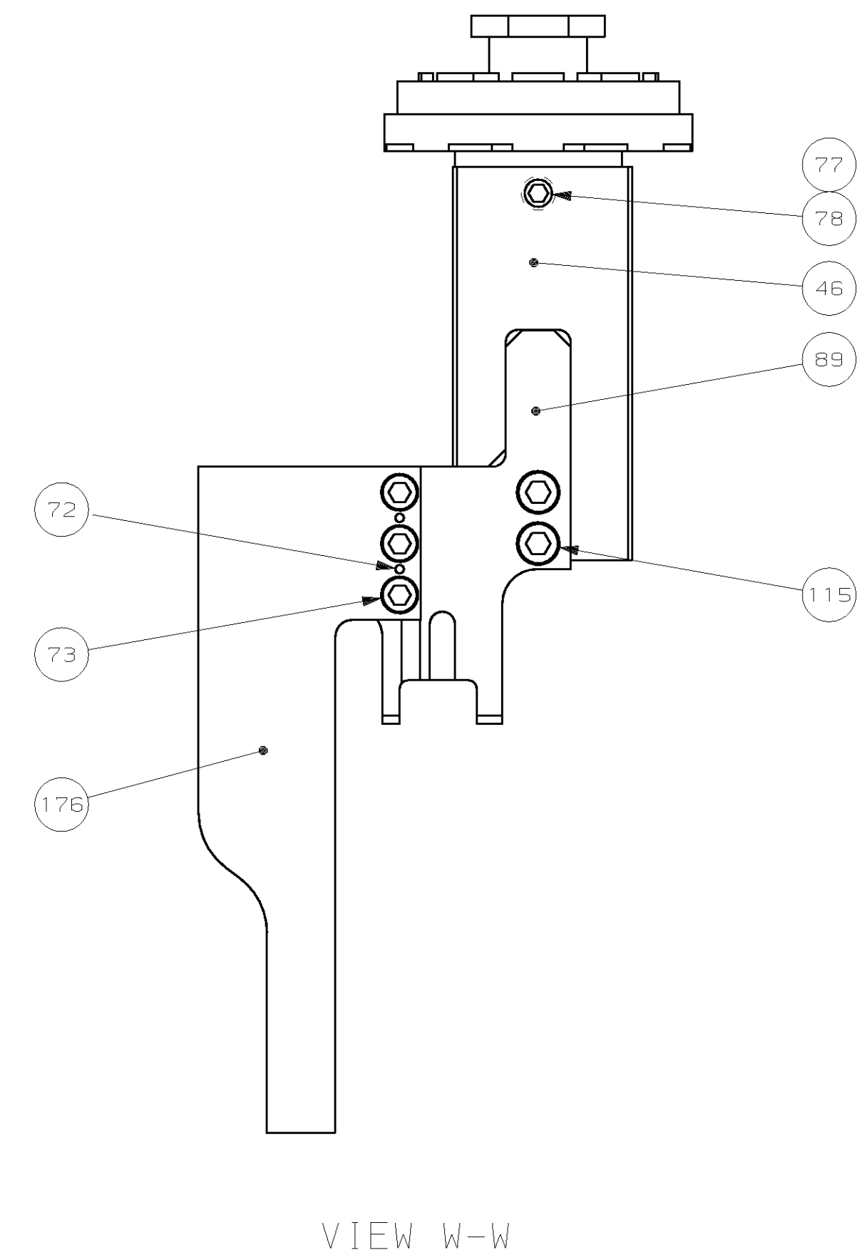
VIEW W-W
