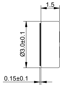
Figure 4. HBO0303C-60 Mechanical Layout
