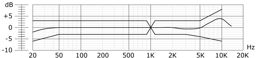
Figure 1. Frequency Response
