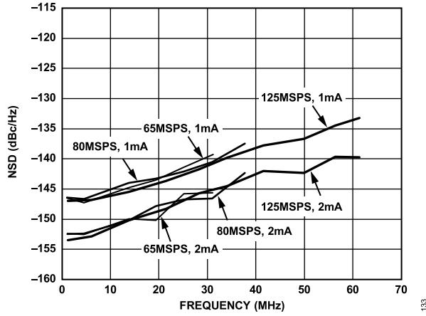
Figure 33. NSD vs. f_{OUT} , f_{LOCK} , and I_{OUTFS} at 0 dBFS
