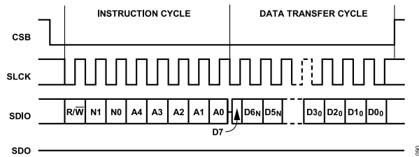
Figure 72. Serial Register Interface Timing, MSB First Read
