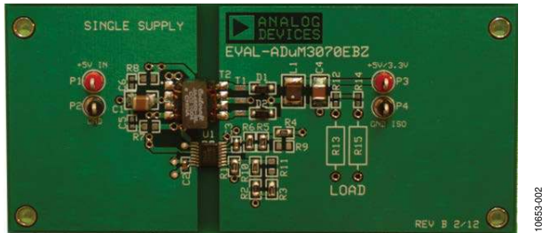
Figure 2. Single Supply Configuration
