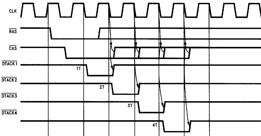
FIGURE 21. DTACK Programmed to Assert from a Negative Edge of Clock
