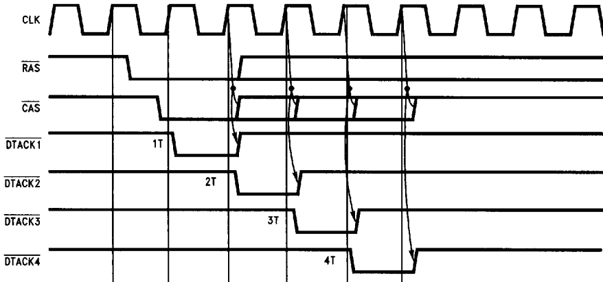
FIGURE 20. DTACK Programmed to Assert from a Positive Edge of Clock
