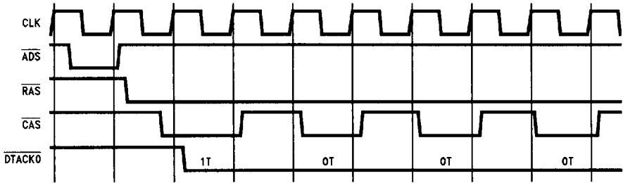
FIGURE 23a. 1T during Opening and 0T during Burst. \overline{DTACK} stays asserted during the burst.
