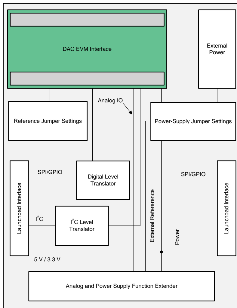
Figure 7. BOOSTXL-DAC-PORT Hardware Block Diagram
