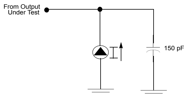
Figure 56. Test Load Diagram
