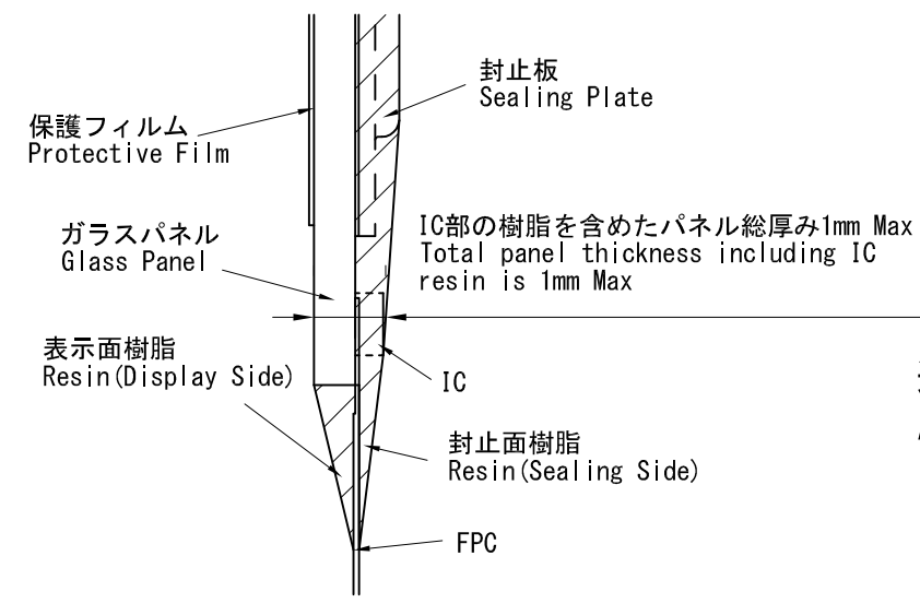
B部拡大図 (10 : 1) B-Portion Magnified Drawing (10:1)
