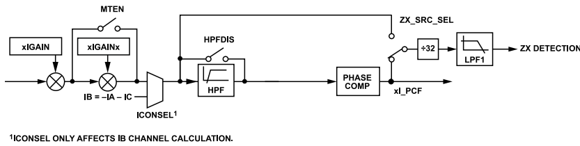
Figure 50. Current Channel Signal Chain Preceding Zero-Crossing Detection
