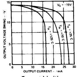
Current Limiting
