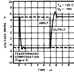
Inverter Pulse Response
