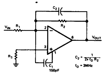
Figure 3. Feedforward Compensation
