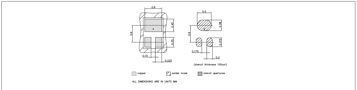
Figure 23 Foot print
