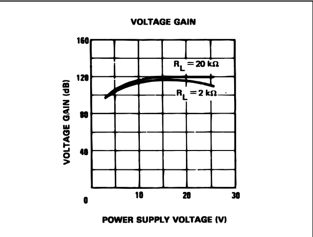
Figure 19. Voltage gain
