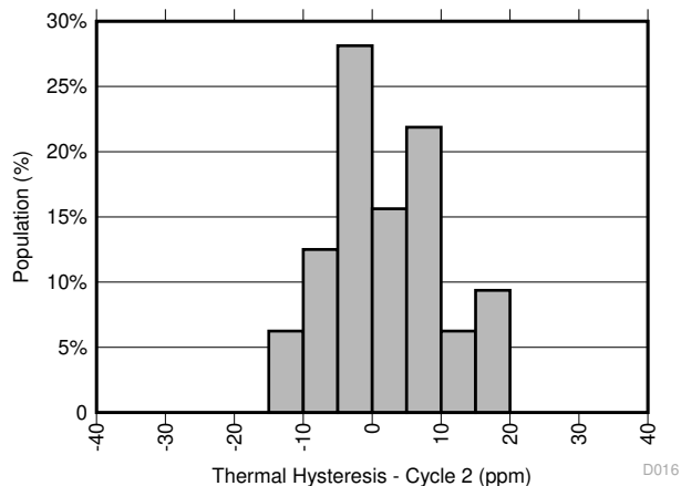
Figure 9-7. Thermal Hysteresis Distribution ( V_{REF} ) - DBV Package (Cycle 2)
