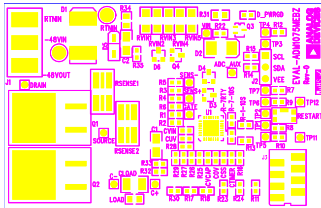
Figure 14. Assembly Top
