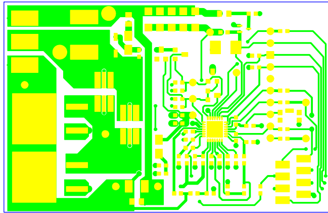
Figure 12. Top Layer
