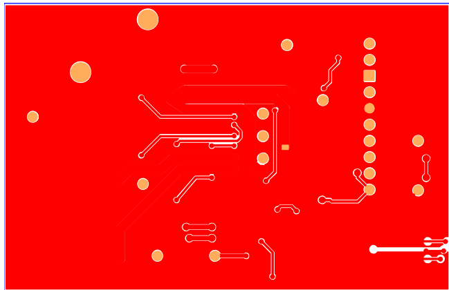
Figure 13. Inner Layer 2
