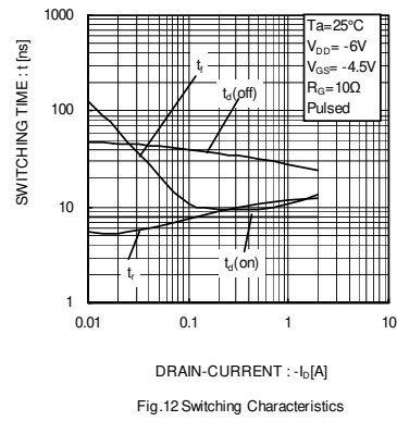
Fig.12 Switching Characteristics
