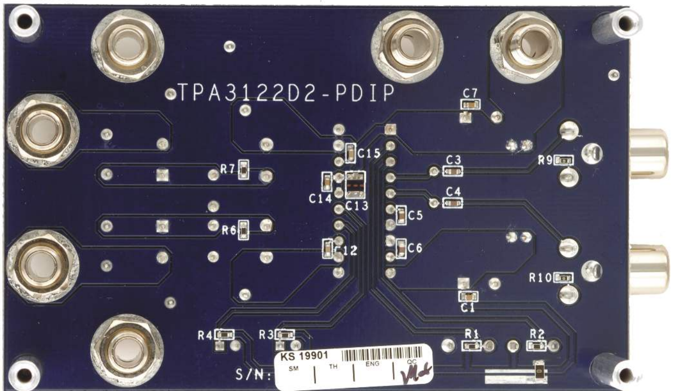
Figure 2. TPA3122D2 Audio Power Amplifier EVM - Bottom View
