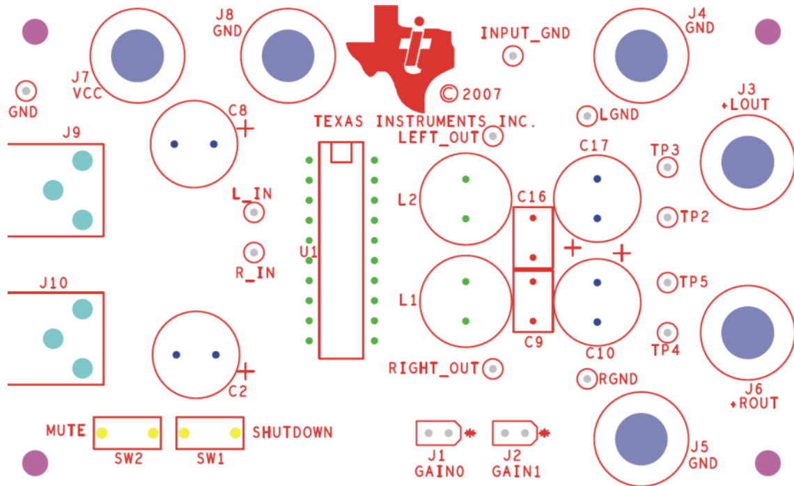
Figure 4. TPA3122D2 EVM – Top Side Layout
