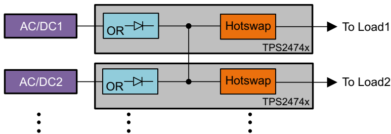
Figure 64. Block Diagram for Systems with Multiple Supplies and Loads
